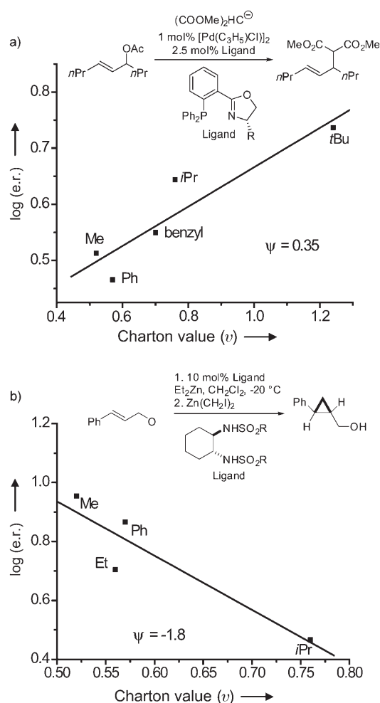
Figure 3. a) Charton plot of Pfaltz's enantioselective Pd-catalyzed allylic allylation using phosphine oxazoline ligands. b) Charton plot of Denmark's enantioselective cyclopropanation with bis(halomethyl)zinc reagents using bis(sulfonamide)-derived chiral diamines.
